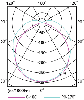
Light Distribution Diagram - 60WP/LED/850/LS EX39 G3 BB 3/1
