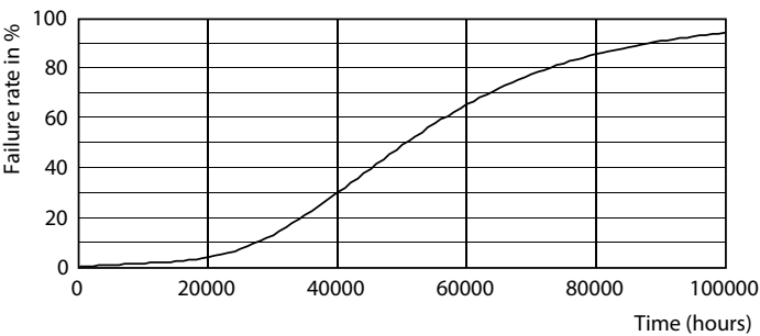
Life Expectancy Diagram - 60WP/LED/850/LS EX39 G3 BB 3/1
