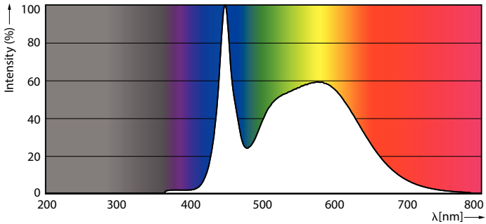
Spectral Power Distribution Colour - 60WP/LED/850/LS EX39 G3 BB 3/1
