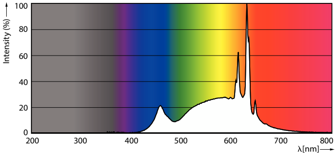
Spectral Power Distribution Colour - LEDBulb 6W B22 930 230V 1PF/6 AU
