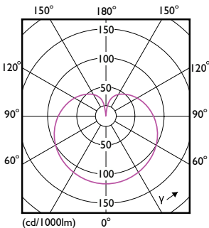
Light Distribution Diagram - LEDBulb 6W B22 930 230V 1PF/6 AU
