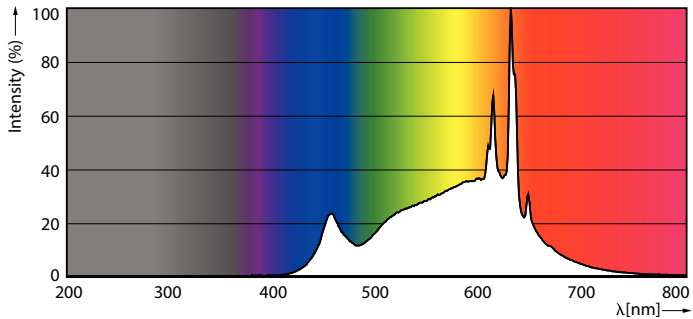
Spectral Power Distribution Colour - LEDBulb 12W E27 930 230V 2PF/3 AU
