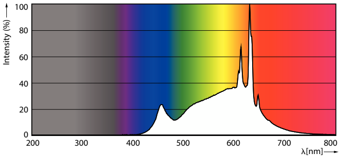
Spectral Power Distribution Colour - LEDBulb 12W E27 930 230V 1PF/6 AU
