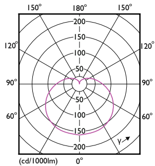
Light Distribution Diagram - LEDBulb 12W E27 965 230V 2PF/3 AU
