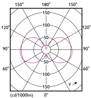
Light Distribution Diagram - MAS VLE LEDCandleDT2.5-25W E14 B35CL G
