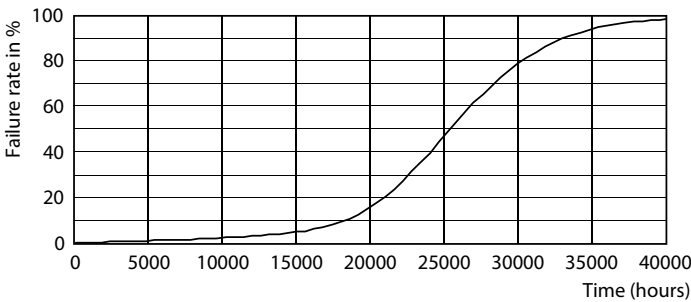
Life Expectancy Diagram - MAS VLE LEDCandleDT2.5-25W E14 B35CL G
