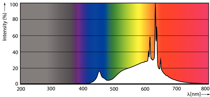
Spectral Power Distribution Colour - MAS VLE LEDCandleDT2.5-25W E14 B35CL G
