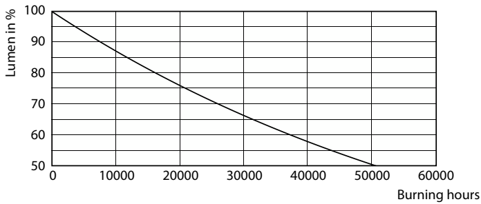
Lumen Maintenance Diagram - MAS VLE LEDCandleDT2.5-25W E14 B35CL G
