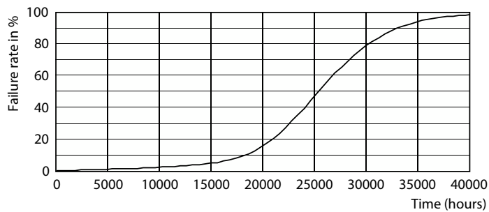
Life Expectancy Diagram - MAS VLE LEDLusterDT2.5-25W E27 927P45CLG
