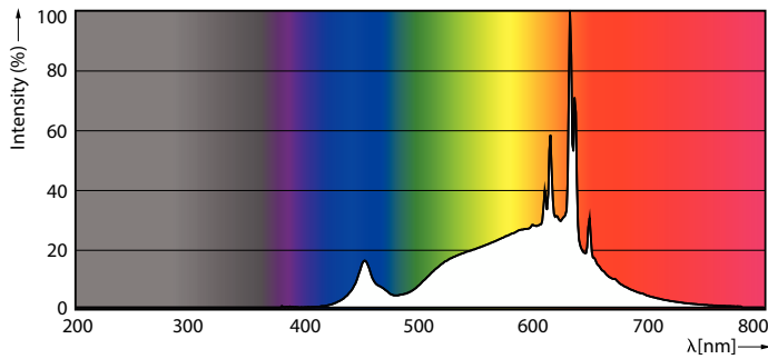
Spectral Power Distribution Colour - MAS VLE LEDLusterDT2.5-25W E27 927P45CLG
