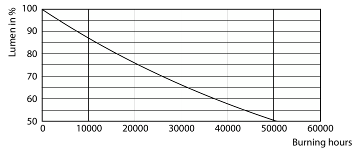
Lumen Maintenance Diagram - MAS VLE LEDLusterDT2.5-25W E27 927P45CLG
