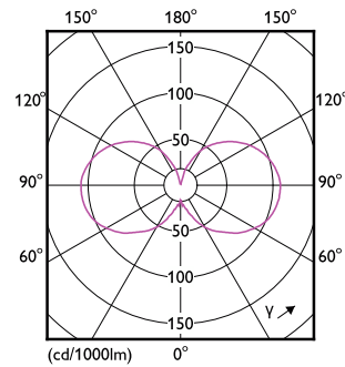
Light Distribution Diagram - MAS VLE LEDLusterDT2.5-25W E27 927P45CLG
