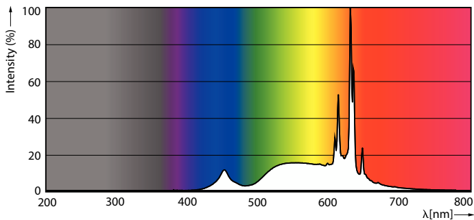
Spectral Power Distribution Colour - MAS VLE LEDCandleDT3.4-40W E27 927B35CLG
