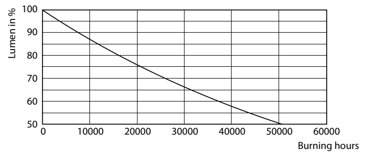
Lumen Maintenance Diagram - MAS VLE LEDCandleDT3.4-40W E27 927B35CLG
