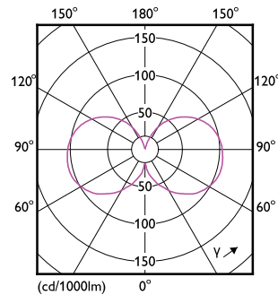
Light Distribution Diagram - MAS VLE LEDCandleDT3.4-40W E27 927B35CLG
