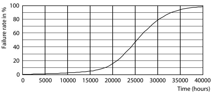
Life Expectancy Diagram - MAS VLE LEDCandleDT3.4-40W E27 927B35CLG
