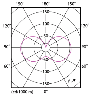
Light Distribution Diagram - MAS VLE LEDLusterDT3.5-40W E27 927P45CLG
