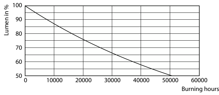
Lumen Maintenance Diagram - MAS VLE LEDLusterDT3.5-40W E27 927P45CLG
