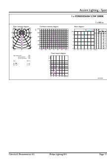
Accent Lighting Spots - 5.5PAR20/LED/F40/930/DIM/G/T20 6/1FB
