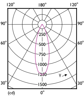
Light Distribution Diagram - 5.5PAR20/LED/F40/930/DIM/G/T20 6/1FB
