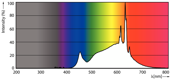
Spectral Power Distribution Colour - 5.5PAR20/LED/F40/930/DIM/G/T20 6/1FB
