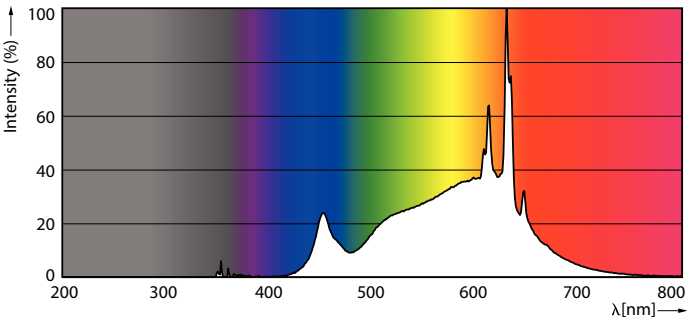
Spectral Power Distribution Colour - 8.5PAR30L/LED/930/F25/DIM/GULW/T20 6/1FB
