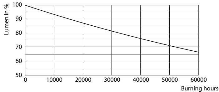
Lumen Maintenance Diagram - LED CLA 40W A60 E27 4000K CL EELA SRT AU
