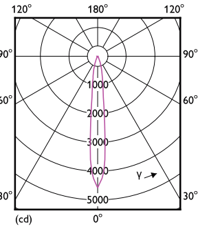
Light Distribution Diagram - MASTER LED 6.5-50W 930 MR16 10D Dim
