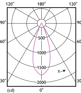
Light Distribution Diagram - 8MR16/LED/830/F35/DIM 12V 10/1FB
