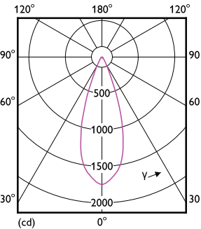
Light Distribution Diagram - MASTER LED 7.5-50W+ 830 MR16 36D Dim
