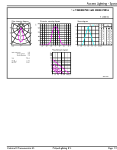
Accent Lighting Spots - MASTER LED 7.5-50W+ 830 MR16 36D Dim
