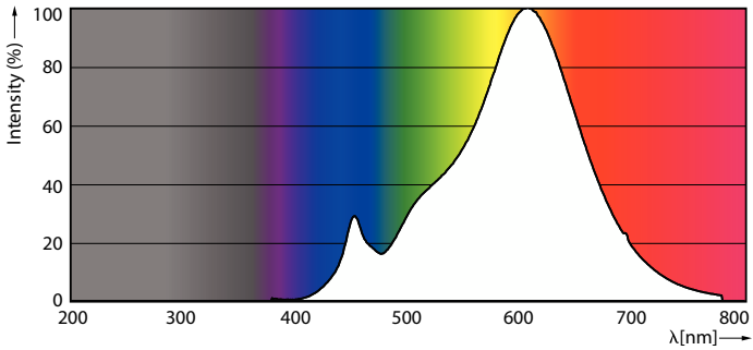
Spectral Power Distribution Colour - MASTER LED 7.5-50W+ 830 MR16 36D Dim
