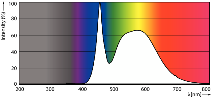
Spectral Power Distribution Colour - 36GC/LED/850/ND E39 BB 6/1
