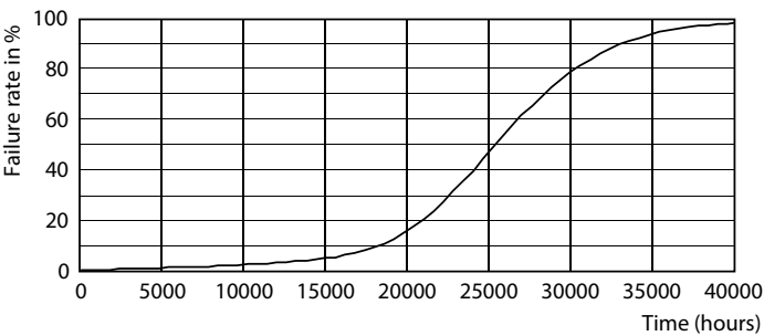
Life Expectancy Diagram - 36GC/LED/850/ND E39 BB 6/1
