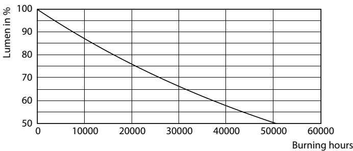
Lumen Maintenance Diagram - 36GC/LED/850/ND E39 BB 6/1
