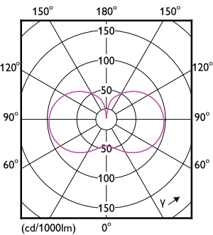
Light Distribution Diagram - 36GC/LED/850/ND E39 BB 6/1
