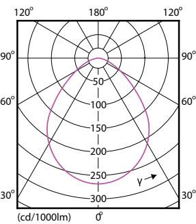
Light Distribution Diagram - Mag L Flood 7W 530lm 30K
