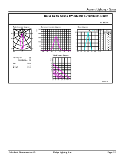
Accent Lighting Spots - RS350 G2 RC Rd D55 4W 30K 24D 1H
