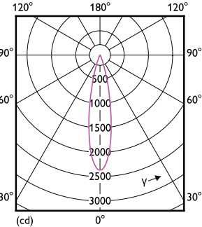
Light Distribution Diagram - RS350 G2 RC Rd D75 4W 40K 24D 1H
