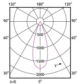
Light Distribution Diagram - RS350 G2 RC Rd D75 7W 30K 36D 1H
