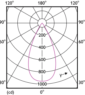
Light Distribution Diagram - RS350 G2 RC Rd D75 7W 30K 50D 1H
