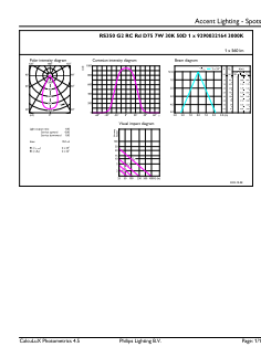
Accent Lighting Spots - RS350 G2 RC Rd D75 7W 30K 50D 1H
