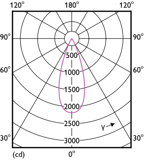
Light Distribution Diagram - RS350 G2 RC Rd D75 9W 40K 36D 1H
