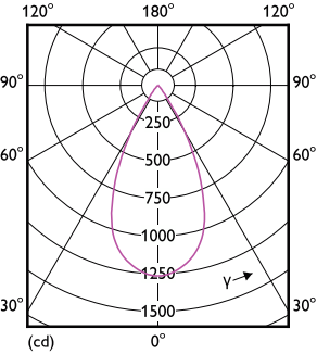
Light Distribution Diagram - RS350 G2 RC Rd D75 9W 40K 50D 1H
