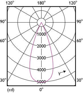
Light Distribution Diagram - RS350 G2 RC Rd D100 20W 30K 36D 1H
