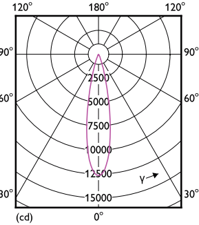
Light Distribution Diagram - RS350 G2 RC Rd D100 20W 40K 24D 1H
