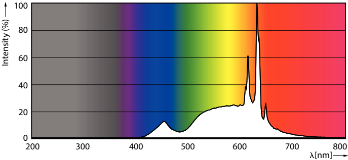
Spectral Power Distribution Colour - CorePro LEDbulb ND 8-60W A60 E27 927
