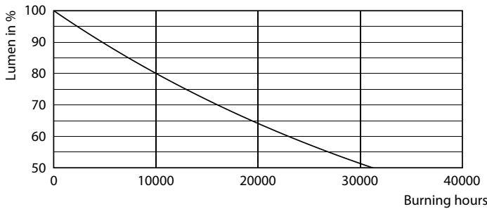
Lumen Maintenance Diagram - CorePro LEDbulb ND 8-60W A60 E27 927
