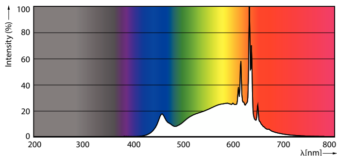
Spectral Power Distribution Colour - 5.5PAR20/COR/F40/930/DIM/P/T20 6/1FB
